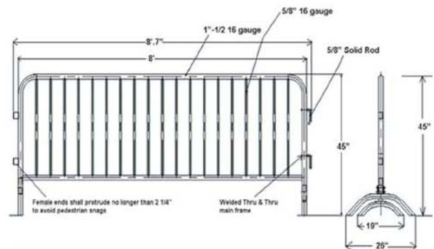
Diagram of Honey Bucket Crowd Control Barricade
